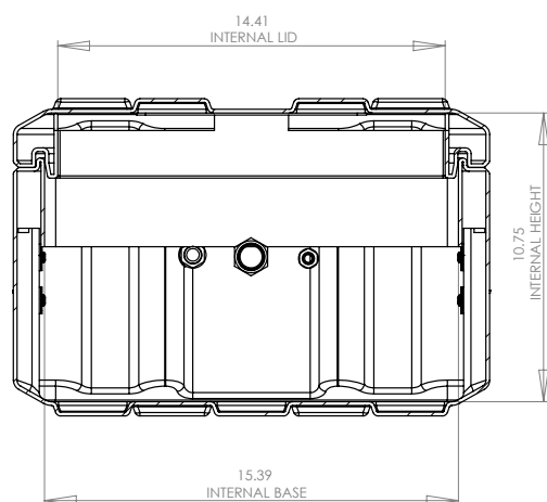
SECTION Y-Y
