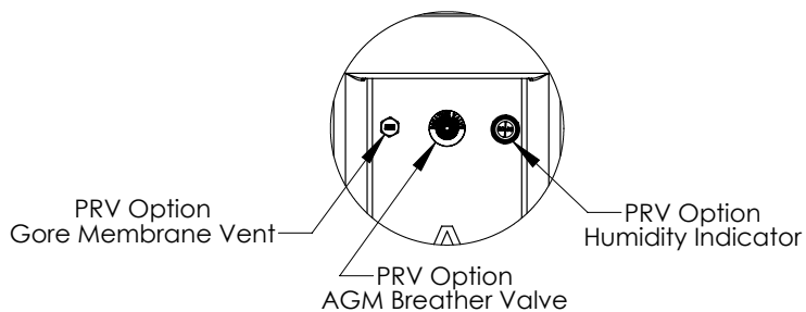
SECTION Y-Y
