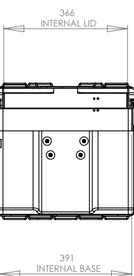
SECTION Z-Z
