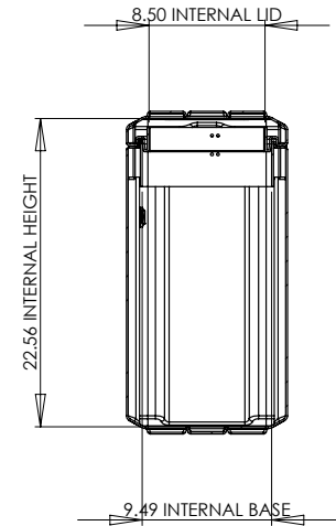
SECTION Z-Z
