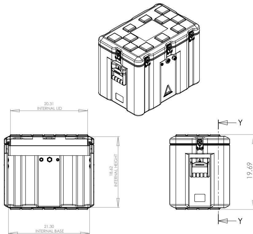
SECTION Y-Y
