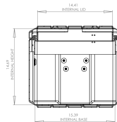
SECTION Z-Z SCALE 1 : 7
