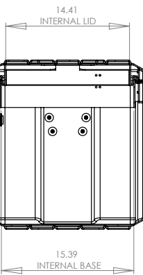
SECTION Z-Z
