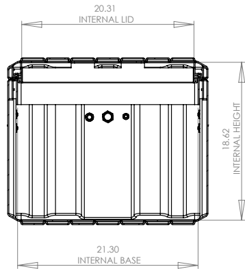
SECTION Y-Y
