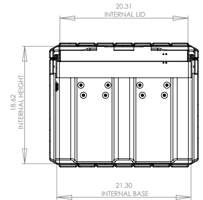
SECTION Z-Z
