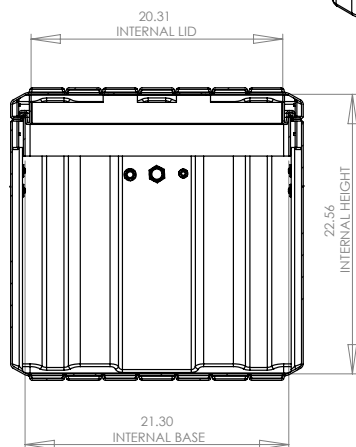
SECTION Y-Y
