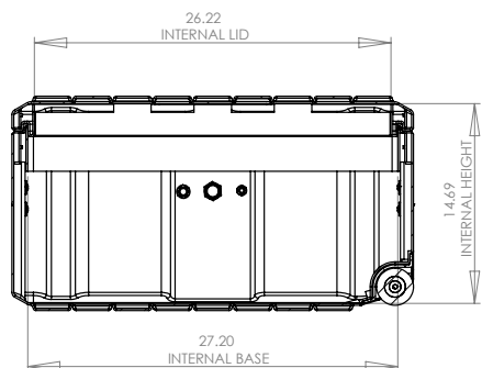
SECTION Y-Y
