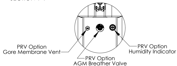
SECTION Y-Y
