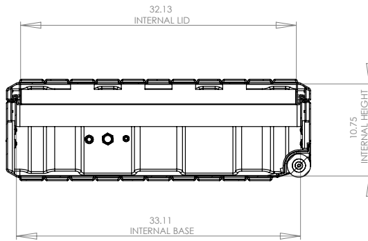
SECTION Y-Y
