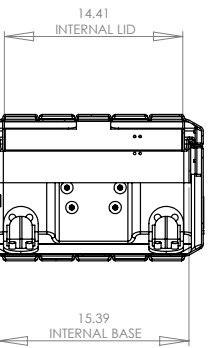
SECTION Z-Z
