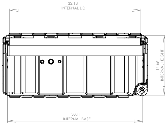
SECTION Y-Y SCALE 1 : 9
