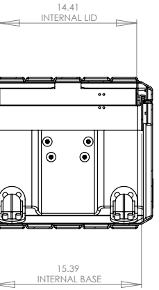
SECTION Z-Z SCALE 1 : 9
