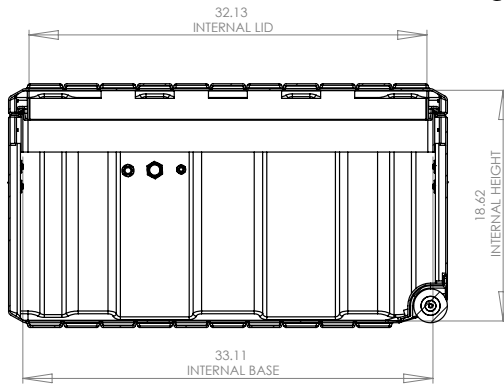
SECTION Y-Y
