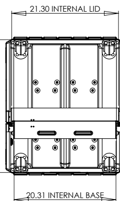
SECTION Z-Z SCALE 1 : 12
