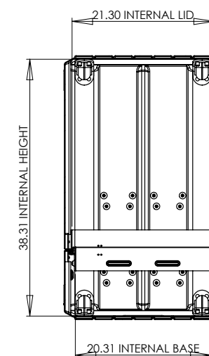
SECTION Z-Z SCALE 1 : 13
