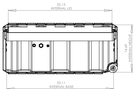
SECTION Y-Y
