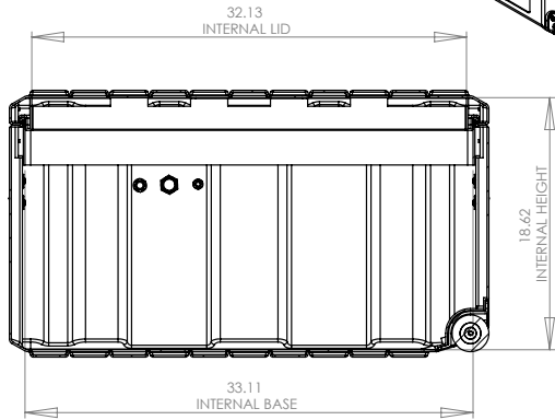
SECTION Y-Y
