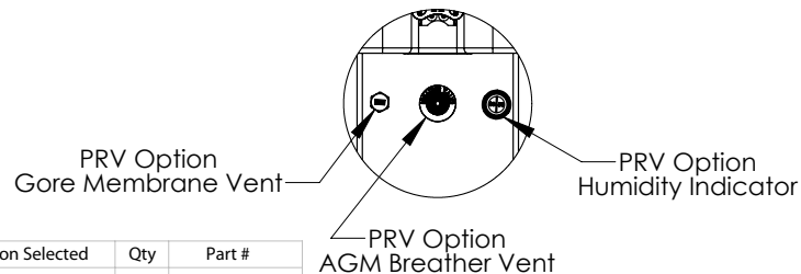
DETAIL A SCALE 1 : 5
