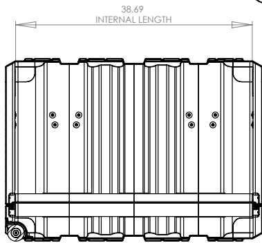
SECTION Y-Y SCALE 1 : 14
