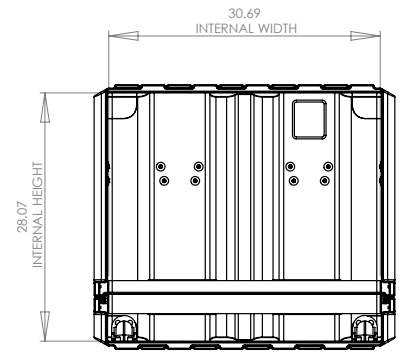
SECTION Z-Z SCALE 1 : 14
