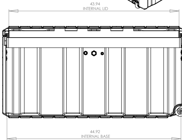
SECTION Y-Y
