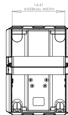
SECTION Z-Z
