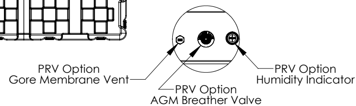
DETAIL A SCALE 1 : 5
